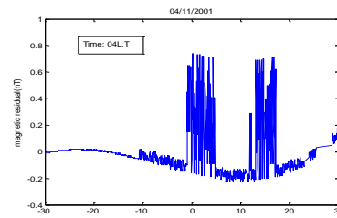
Figure 8a. Two signatures are seen on latitudes; 0 0 and 15 0 .
