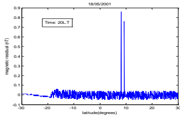
Figure 5b The signature is observed on latitude 9 0 .
