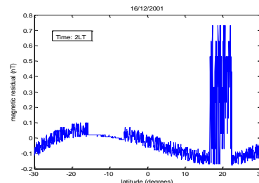
Figure 9a. Shows a magnetic residual on latitude 20 0
