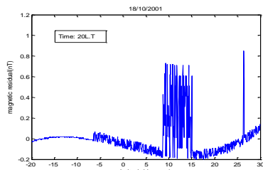
Figure 7c. Two magnetic residuals are observed on latitudes 10 0 and 26 0 .
