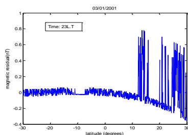
Figure.1a The magnetic residual is seen on various latitudes; 11°, 21° and 29°
