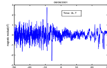
Figure 6b. A magnetic signature of \pm 2.8nT on latitude -7 0 and -10 0 .
