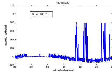
Figure 7b. The signatures are observed on various latitudes; 9 0 , 13 0 , 25 0 and 29 0 .
