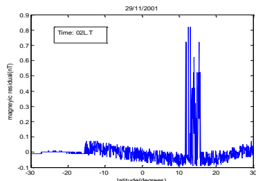
Figure 8b. A magnetic signature is observed on latitude 15 0 .
