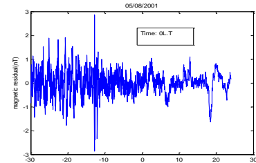
Figure 6a. The signature is observed on latitude -12 0 .
