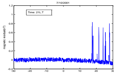
Figure 7a. Magnetic residuals on various latitudes; 19 0 , 25 0 , 28 0 .
