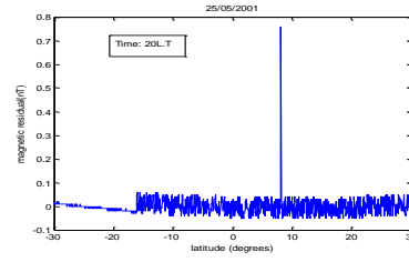
Figure 5e. A distinct signature is recorded before midnight on latitude 9 0 .
