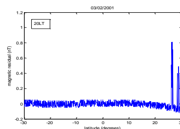
Figure. 2a The magnetic signature is on the northern hemisphere on an latitude 28°.
