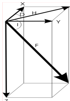
Figure.1 Cartesian components of the geomagnetic elements, x-North, East (M. Kelley), z-vertically downward.
