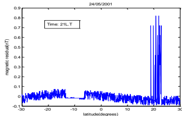
Figure 5d. The magnetic signature is observed on latitude 20 0 .
