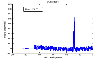
Figure 5c. The signature is observed on latitude 15 0 .
