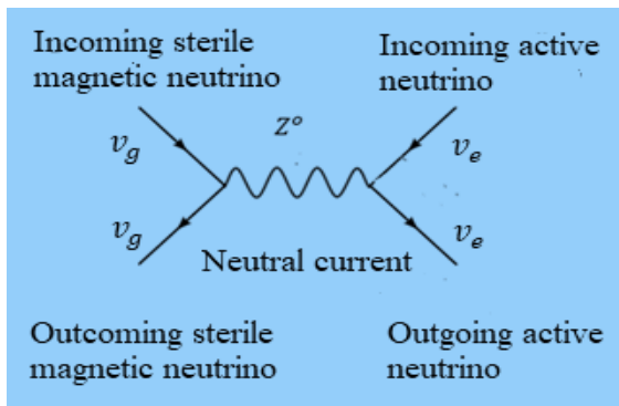
a) A sterile magnetic neutrino of dark matter passing close to an active neutrino of ordinary matter does not disturb the latter and generates no creation of particles, the neutrinos themselves being simply deflected.
