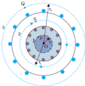
Fig 4. The magnetic field in the open space inside (point P) and exterior to the toroid (point Q) is zero. The field B inside the toroid is constant in magnitude for the ideal toroid of closely wound turns. The direction of the magnetic field inside is clockwise as per the RH thumb rule for circular loops [122].
