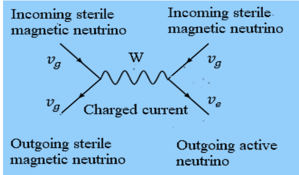
a) We can consider that a weak positive current ( W^+ ) transforms a sterile magnetic neutrino into an active neutrino on the right side.
