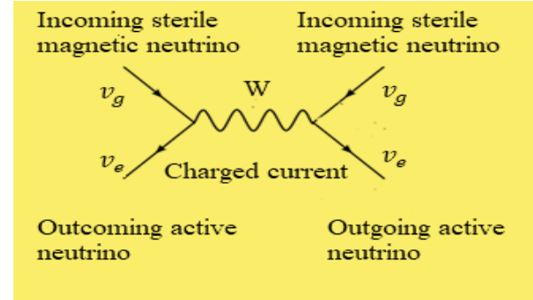
b) We can consider that the weak charged currents flow in both directions ( W^\pm ) and the sterile magnetic neutrino is transformed into active neutrino on the left side while the sterile magnetic neutrino is also transformed into active neutrino on the right side.
