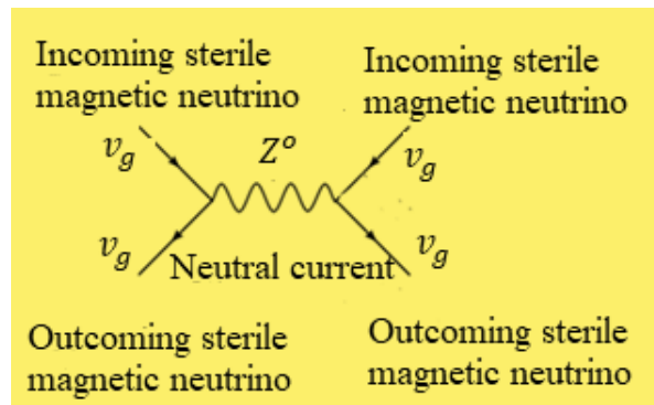
b) A sterile magnetic neutrino of dark matter passing close to another sterile magnetic neutrino of dark matter does not disturb the latter and does not generate any particle creation, the neutrinos themselves being simply deflected.
