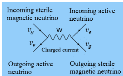
a) A weak charged currents circulate in both directions W^\pm simultaneously, transformed into an active neutrino on the left and right side.
