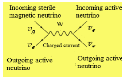
b) We can consider that a weak negative current W^- transforms a sterile magnetic neutrino into an active neutrino on the left side.
