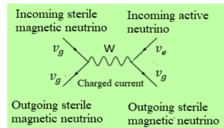
c) We can consider that a weak positive current W^+ transforms an active neutrino into a sterile magnetic neutrino on the right side.
